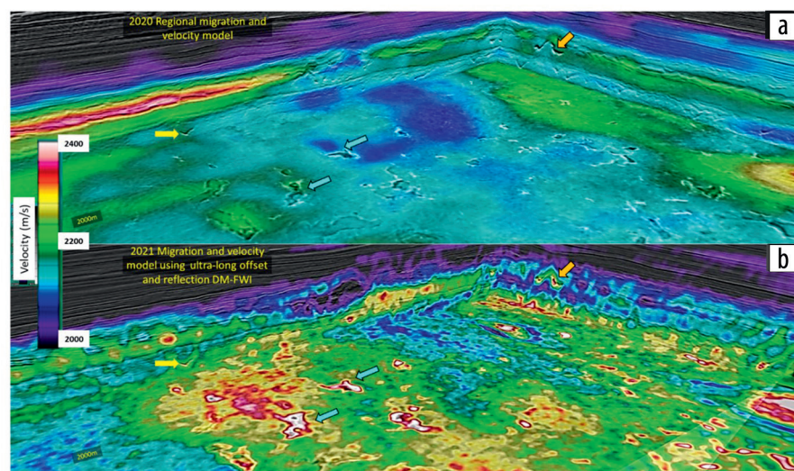
Figure 6. Chair diagram of North Sea OBN FWI-based velocity models overlain atop final migrated images. Both model building efforts included well calibration and anisotropy updates. (a) 2020 regional processing. (b) 2021 detailed processing using DMFWI.
