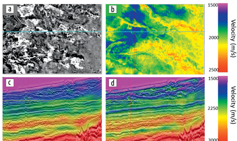
Figure 11. Gabon NAZ DMFWI example. (a) Depth slice of intermediate migration ( z = 2.4 km) illustrating shallow sediment complexity. Blue horizontal line indicates approximate location of crossline shown in (c) and (d). (b) Depth slice of final velocity model after DMFWI update ( z = 2.4 km). (c) Initial model overlaid atop crossline migrated using initial model. (d) Final (DMFWI-updated) model overlaid atop crossline migrated using final model.
